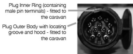
Fig. 1 - 13 Pin Plug
